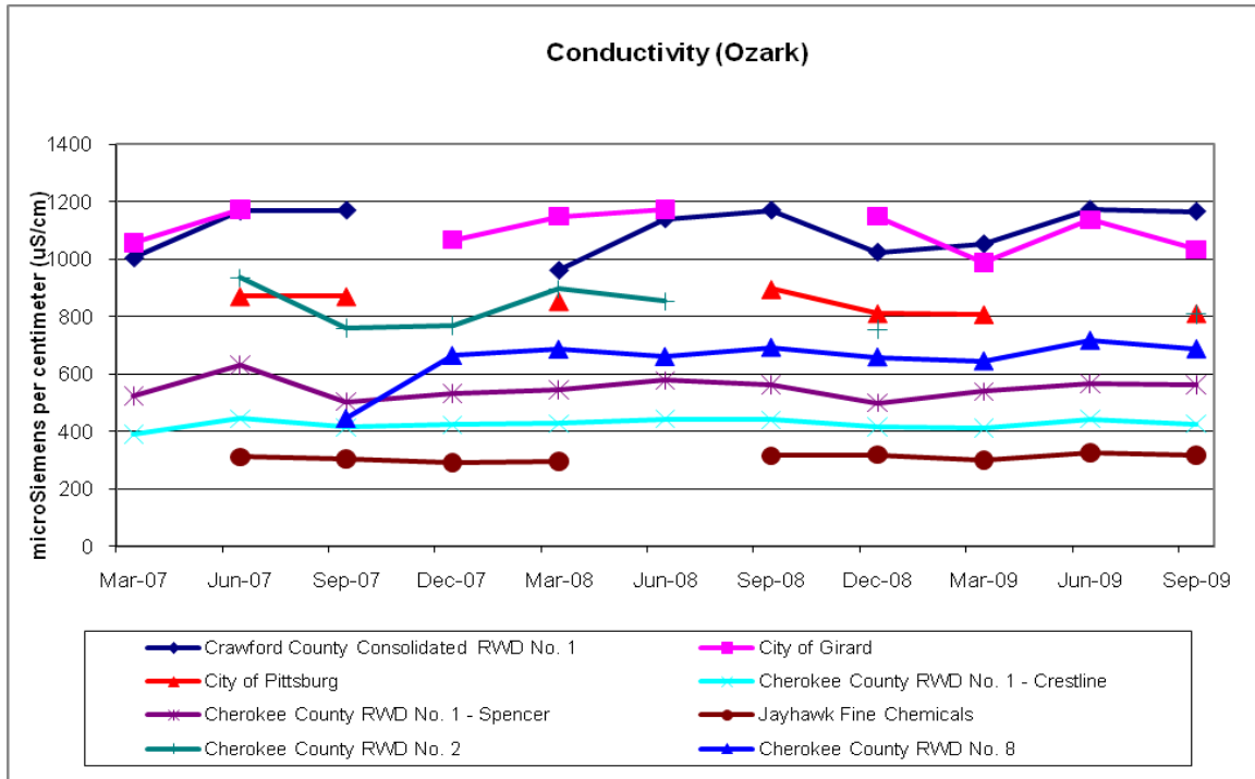
Figure 3: Ozark Aquifer Conductivity
