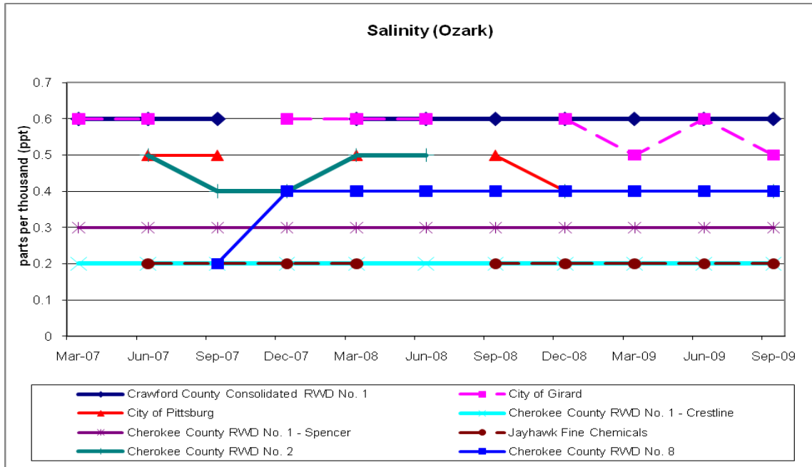
Figure 1: Ozark Aquifer Salinity
