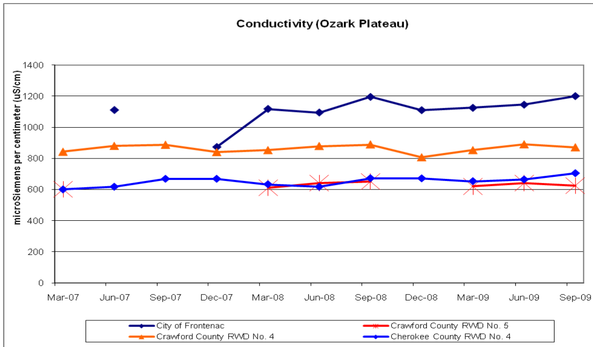
Figure 4: Ozark Plateau Aquifer Conductivity
